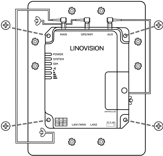
LINOVISION IOT-R32W
