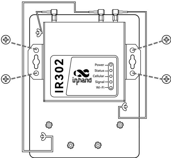
InHand IR302
