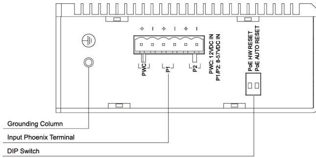
Figure 2-2 Schematic diagram of the side panel of the switch
