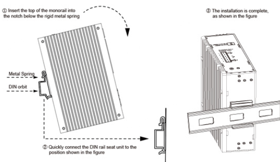
Figure 4-1 Schematic diagram of industrial machine guide rail installation1
