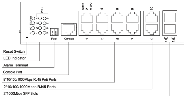
Figure 2-1 Front panel of the Switch
